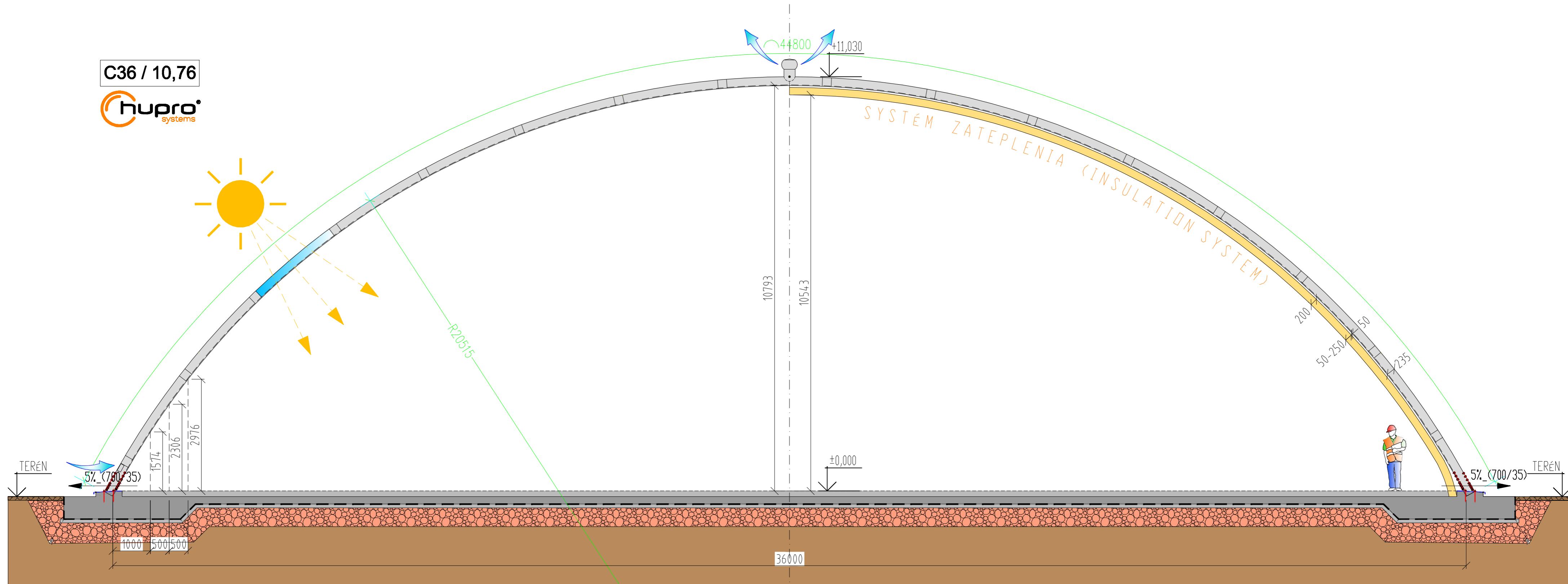
ORIENTAČNÝ TVAR ZAKLADANIA (ORIENTATION FORM OF FOUNDING)
